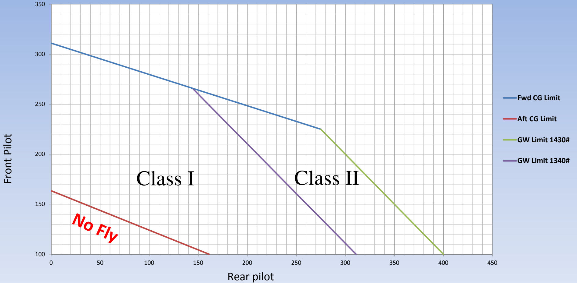
N964E Pilot Weight Limits
